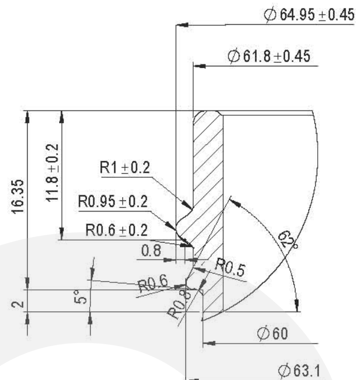
FINISH DETAIL SECTION A-A SCALE 3:1
