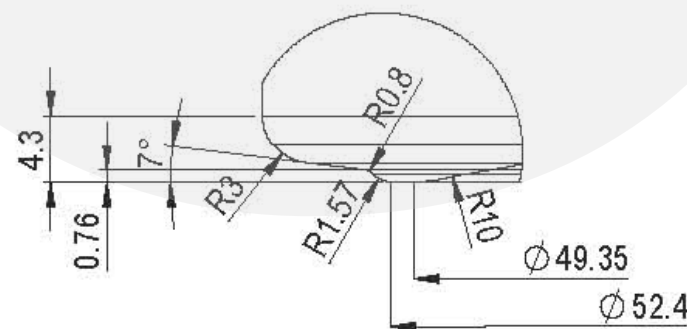
DETAIL C SCALE 2:1
